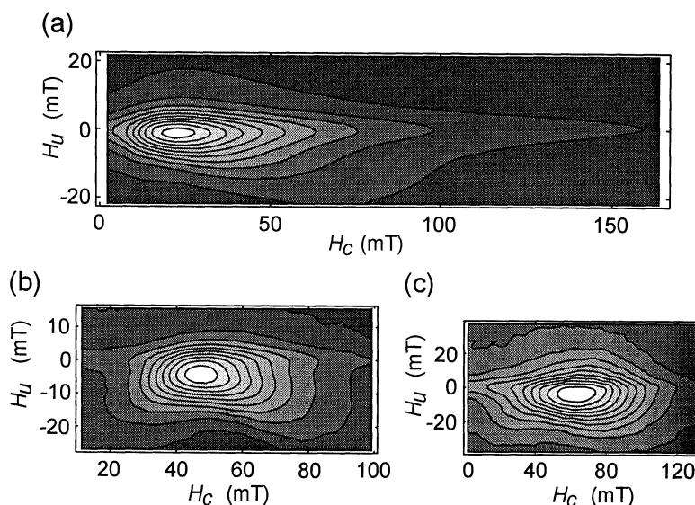
Figure 4. FORC diagrams for geological samples containing interacting SD particles. (a) FORC diagram for sample CRB-15 from the Columbia River Basalt (see text). (b) FORC diagram for sample CRP-1-145.46 from Miocene glaciomarine sediments, Antarctica (see text). (c) FORC diagram for sample BV1348 from Pleistocene lake sediments, northern California (see text).
